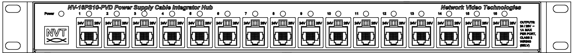
NV-16PS10-PVD POWER SUPPLY CABLE INTEGRATOR HUB FRONT VIEW
