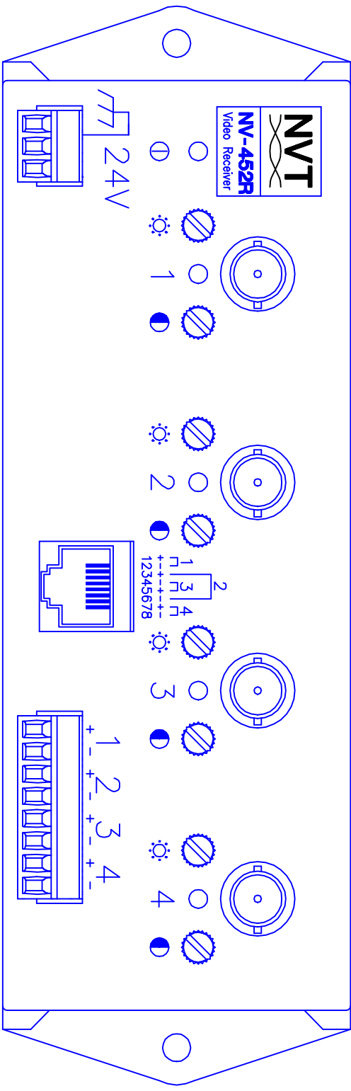
NV-452R TOP VIEW
